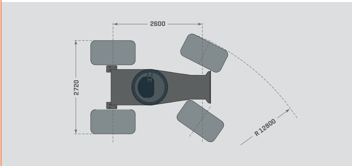
AXLE ZF 3060, TIRE 710 / 26,5"
