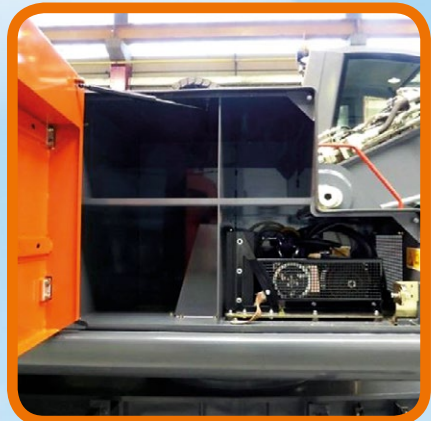
Compressor unit for electric heating and climate control system
